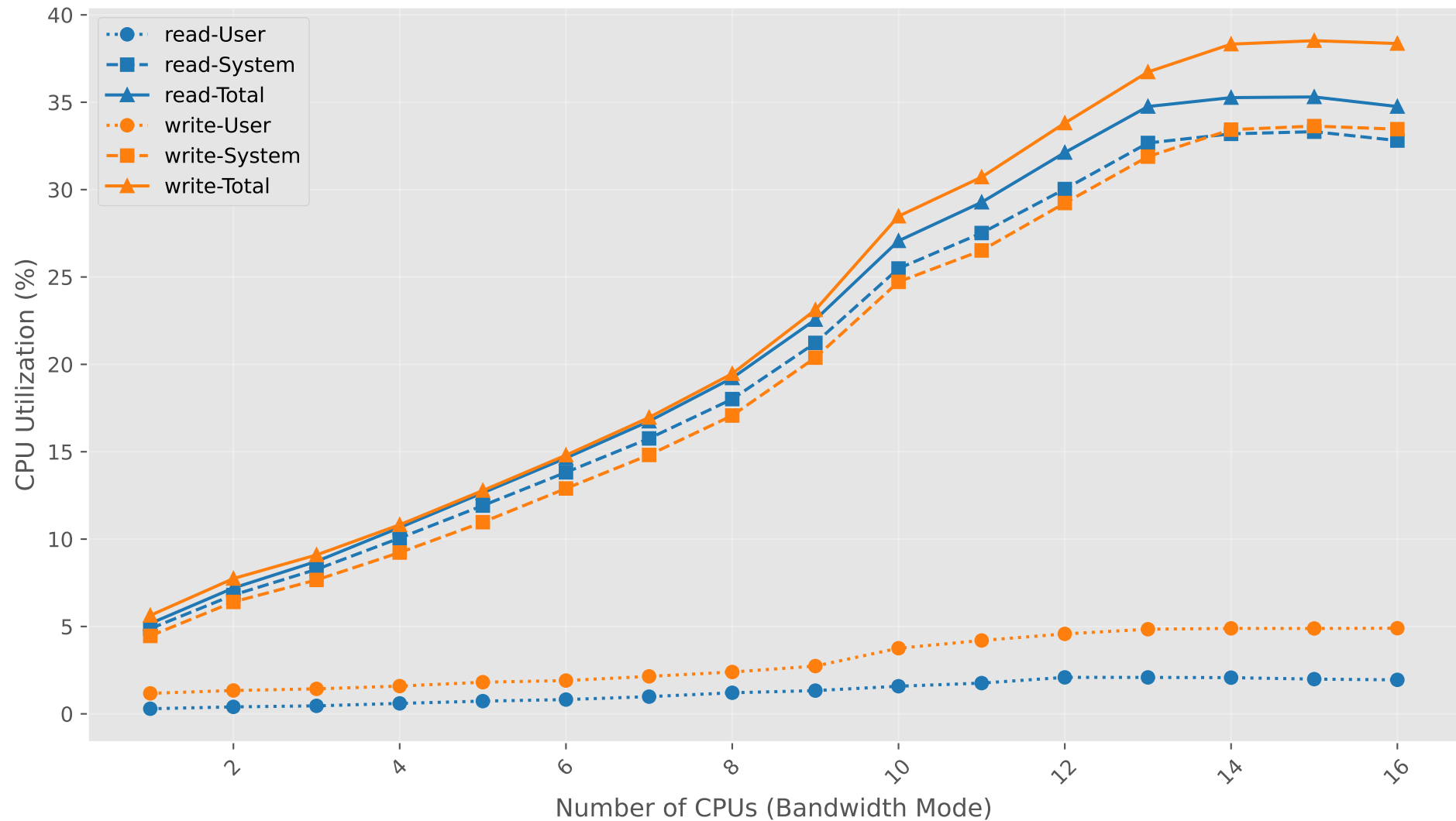
CPU Total vs Number of CPUs (Bandwidth Mode)
